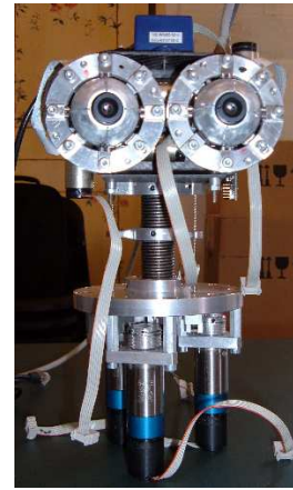
Fig. 4. Prototype of robot head with spring-based neck.
