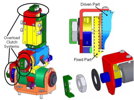
Fig. 8. Clutch based overload protection system.
