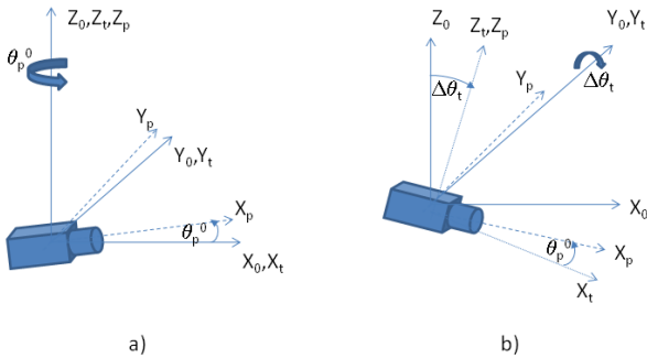
Fig. 2. The geometry of the system before (a) and after (b) the prospective motion.
