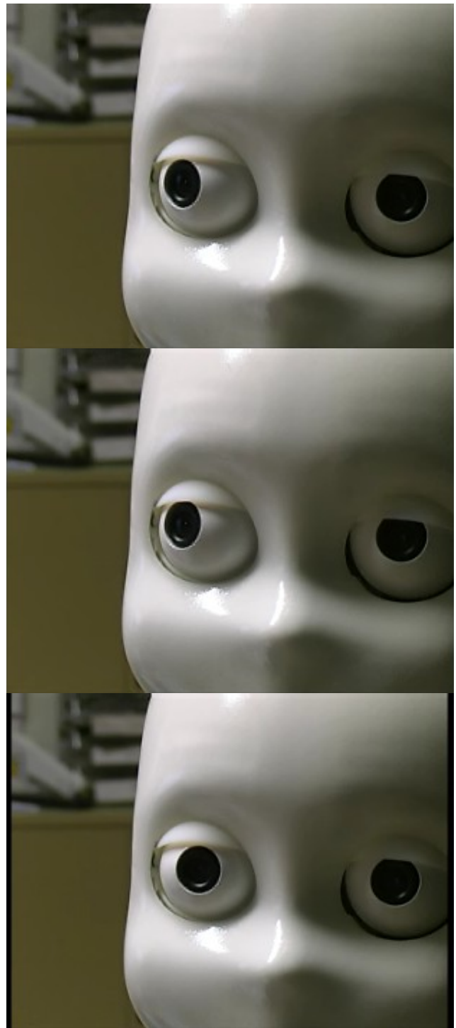
Fig. 4. Sequence of motions required to calibrate the eye. Top: right eye position at startup. Middle: right eye position after prospective tilt motion. Bottom: right eye position after calibration
