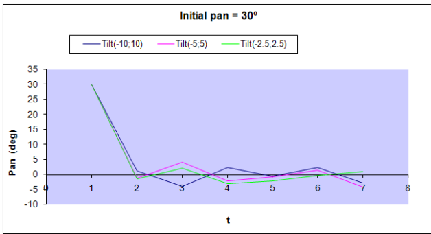
Fig. 7. Evolution of the pan angle for an iterative application of the calibration method. Different colors represent different prospective motion amplitudes.
