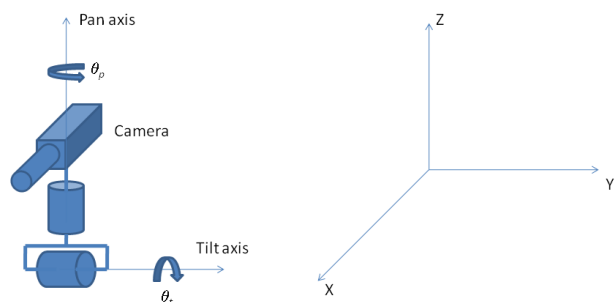
Fig. 1. Left: the kinematics structure of the pan-tilt system considered in this paper. Right: the adopted orientation for all the involved coordinate frames.
