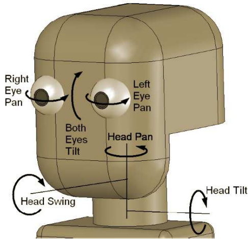
Fig. 3. Kinematics of the iCub robot head used in the tests
