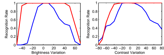
Figure 2. Recognition rates with brightness (left) and contrast variation (right) for the probabilistic rigid model (red) and template matching (blue).
