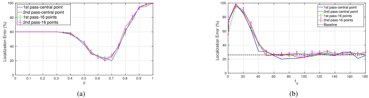
Fig. 6: Localization Performance: (a) in function of the threshold applied to the segmentation mask with a fixed fovea size f_0 = 70 ; (b) in function of the fovea size f_0 where the threshold applied to the segmentation mask was set to \theta = 0.7 since it results in a minimum localization error.
