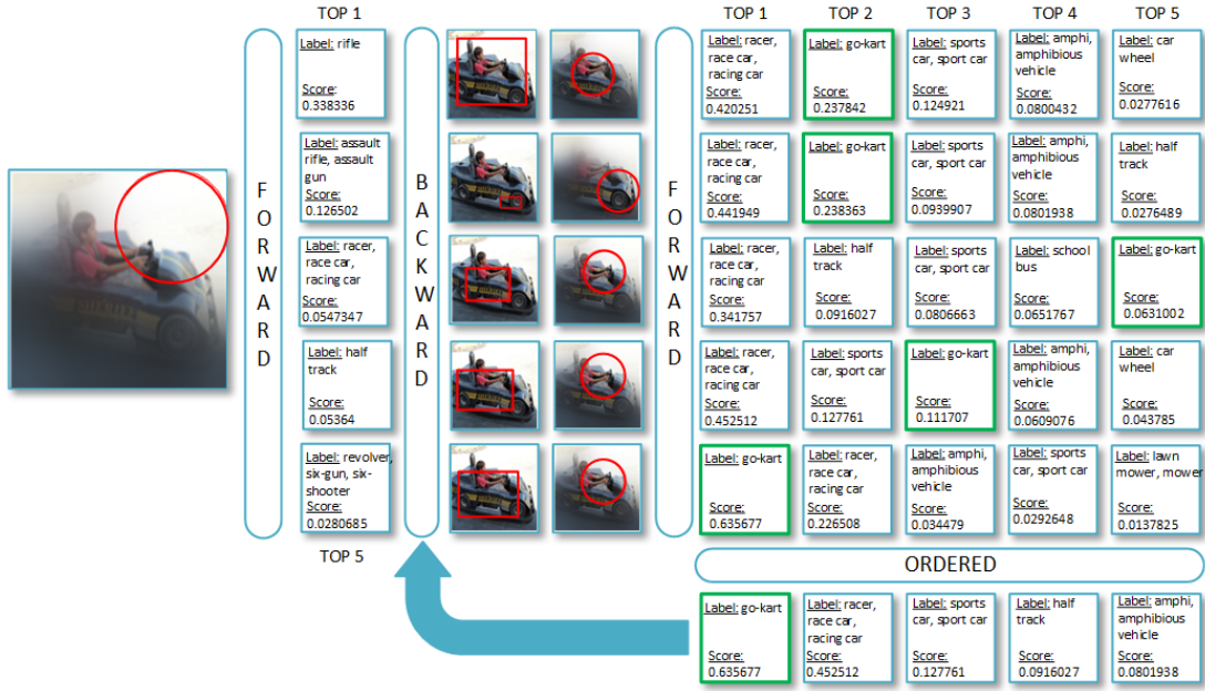
Fig. 3: Schematic of our iterative refinement model of object detection. First a foveated resized image is loaded into the network to predict the top-5 class labels through a feed-forward pass. Then for each class label, it is computed each bounding box with a top-down back-propagation according to the threshold selected. Then we apply a second foveation centered in each bounding box found and predict again the top 5 class labels with a feed-forward. Given this 25 labels with confidences associated we sort them in descending order, not choosing repeated labels and pick as final solution the top-5. Iteratively we to a re-localization according to those labels with a feedback pass. In our work we only considered two iterations. The red rectangles represent the bounding boxes that contain all pixels above the specified threshold, in this case the threshold was 0.75. The red circles represent the focused area simulating the fovea, that was set to f_0 = 60 in this case. The ground truth label of the input image is go-kart.
