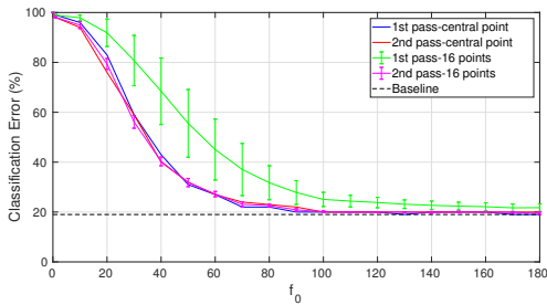
Fig. 5: Classification Performance in function of the fovea size f_0 with \theta = 0.7 . The baseline was computed with f_0 = 227 (the resolution of the input image) to simulate an input image without any blur corresponding to minimum error
